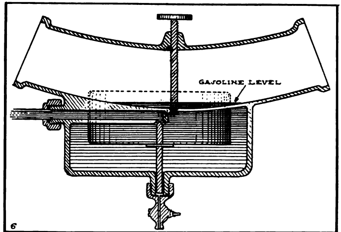
Fig. 6—Showing the accumulation of gasoline in the pan of the depression chamber, as the result of priming.
